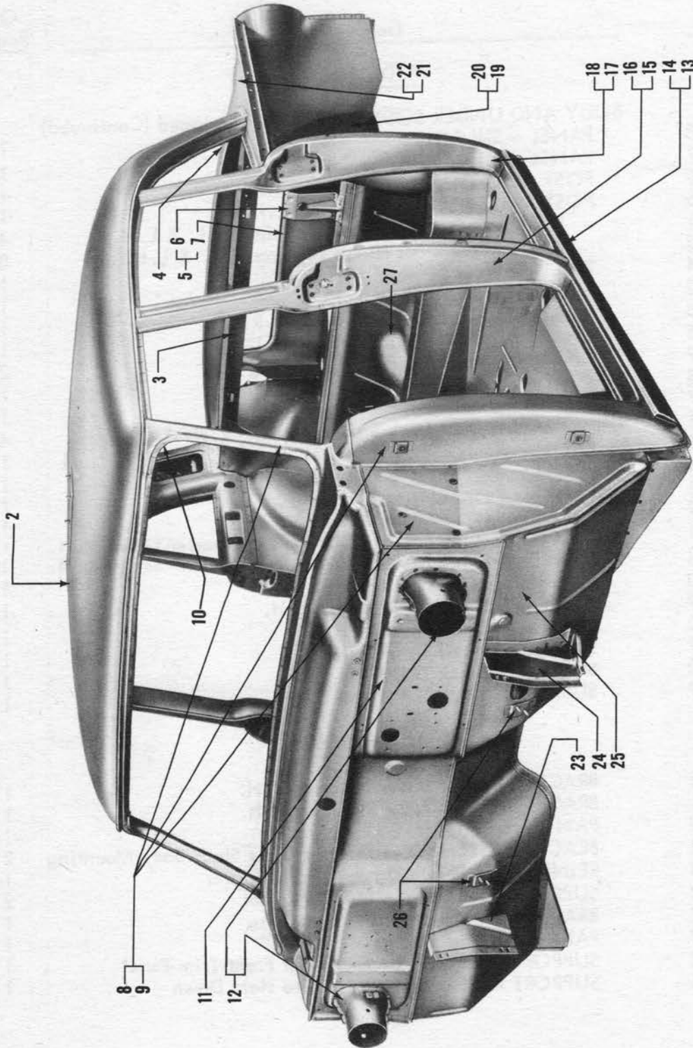
#1—BODY AND UNDERBODY ASSEMBLY
