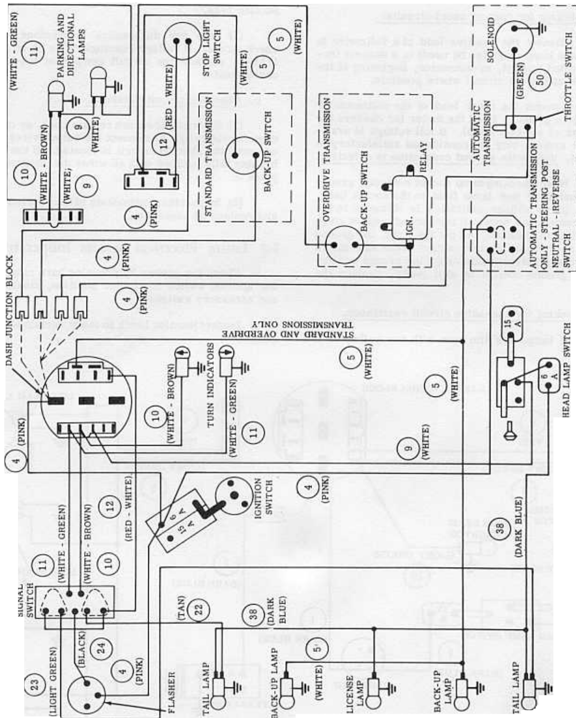
Fig. 2 - Tail Lamp, Back-Up Lamp, and License Lamp Wiring
